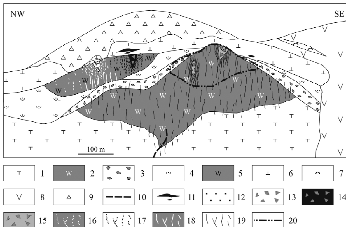
Fig. 1. An idealized geological section through the Madneuli deposit. 1 - Tuff of the first package; 2 - Lower silica-rich body; 3 - Breccia-conglomerate of the second package; 4 - Tuff of the third package; 5 - Upper silica-rich body; 6 - Tuff of the fourth package; 7 - Tuff of the fifth package; 8 - Extrusive body; 9 - Ignimbrite; 10 - Inferred fault; 11-12 - Syngenetic stratiform ores: 11 - Barite-sphalerite-pyrite; 12 - Quartz-barite; 13-15 - Epigenetic breccia ores: 13 - Quartz-barite; 14 - Barite-sphalerite-pyrite; 15 - Quartz-pyrite-chalcopryrite; 16-19 - Epigenetic vein-disseminated ores: 16 - Quartz-barite; 17 - Barite-sphalerite-pyrite; 18 - Chalcopryrite-sphalerite; 19 - Quartz-pyrite-chalcopryrite; 20 - Contour of oxidized ores.
