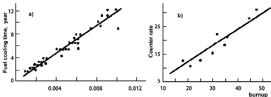
Fig. 2. a) Dependence of fuel cooling time vs I/I_0 , where I - Intensity of ^{137}\text{Cs} \gamma -radiation, I_0 - total intensity of \gamma - radiation); b) Relation between count rate of \gamma -radiation and burnup factor.
